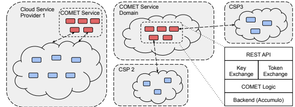
Figure 1. COMET Metadata service architecture
