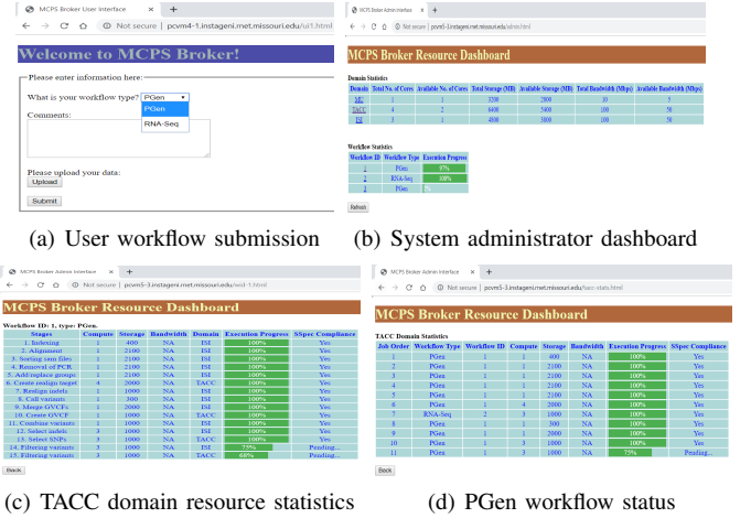
Fig. 2: MCPS Broker User Interface
