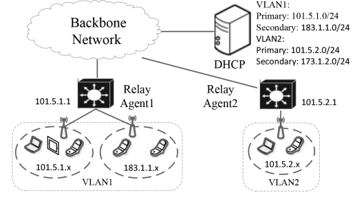
Fig. 1: The widely deployed DHCP architecture.
